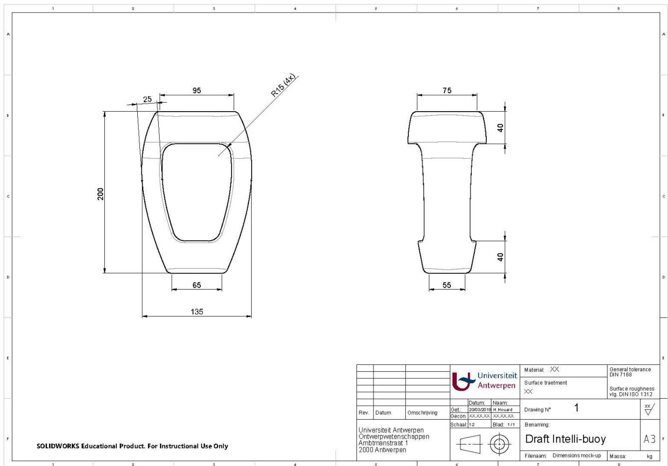
Figure 36: Dimensions
