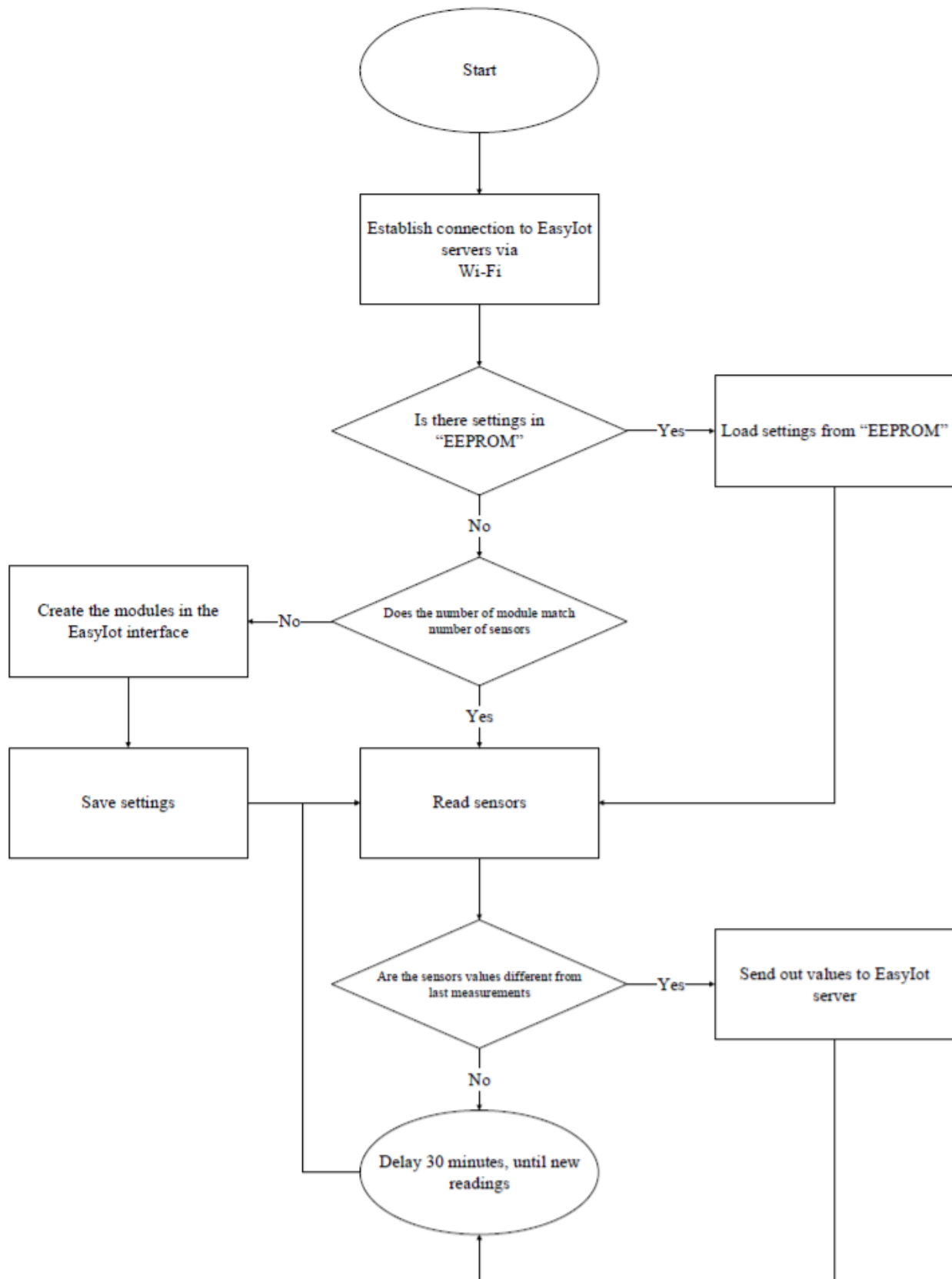
Figure 31: Flowchart of the code
