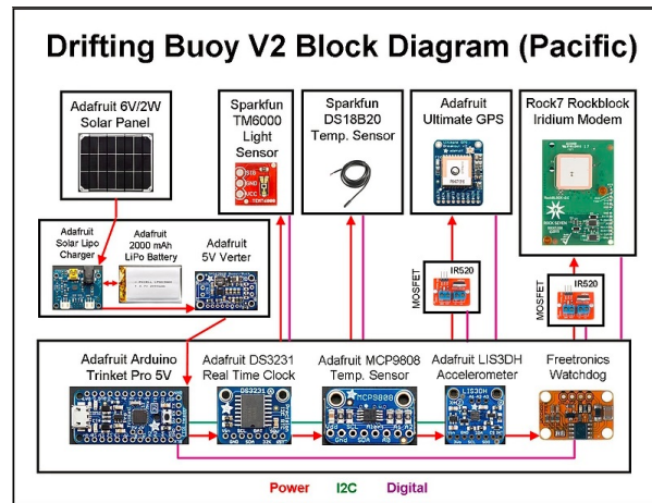
Figure 4: Block diagram [18]
