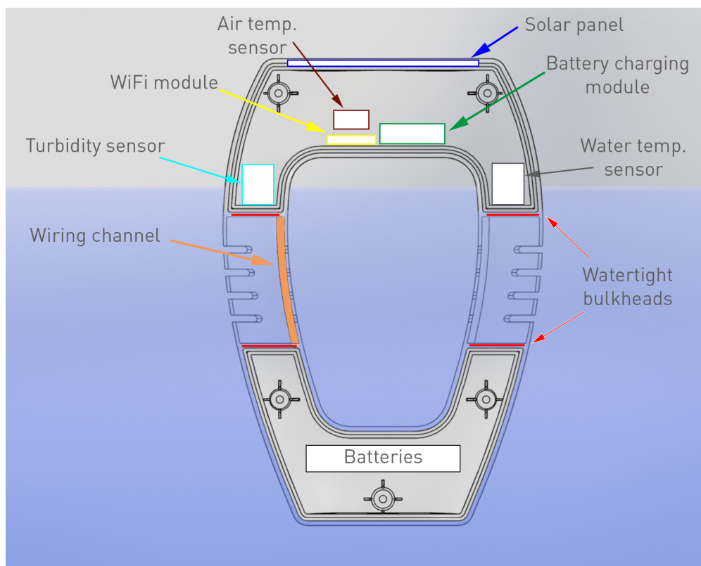
Figure 46: Positioning of the components
