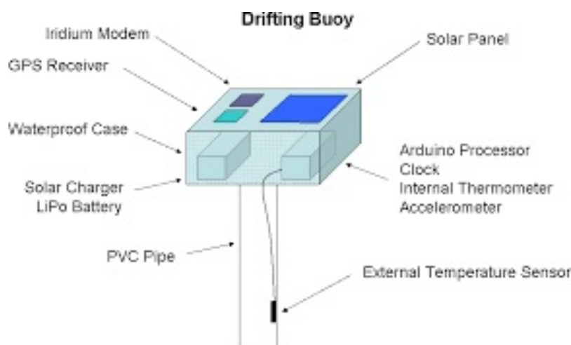
Figure 3: Diy buoy [16]
