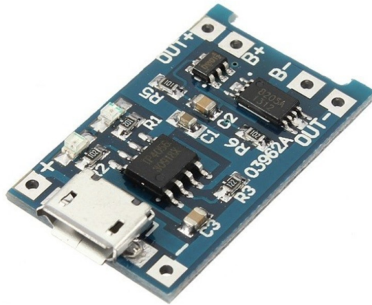
Figure 42: Battery charger module component [84]
