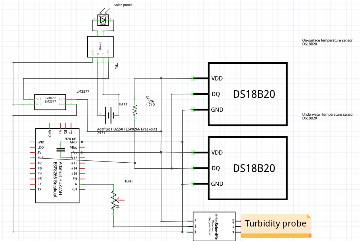
Figure 38: Electrical schematic
